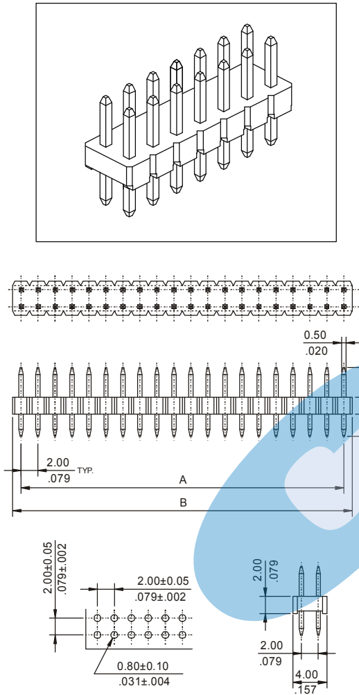
RECOMMENDED HOLE PATTERN
