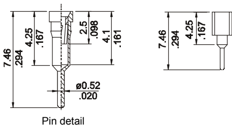
Pin detail
