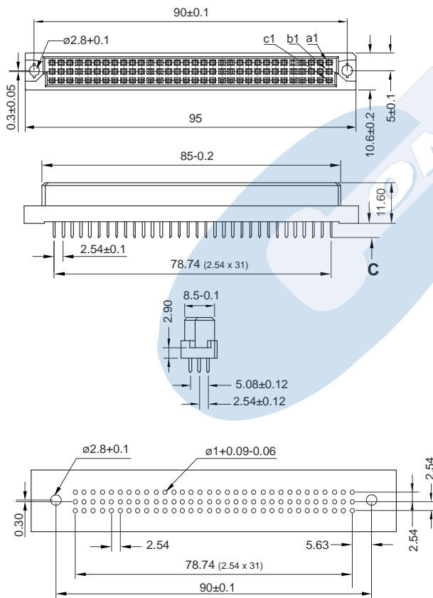
RECOMMENDED PCB HOLE LAYOUT
